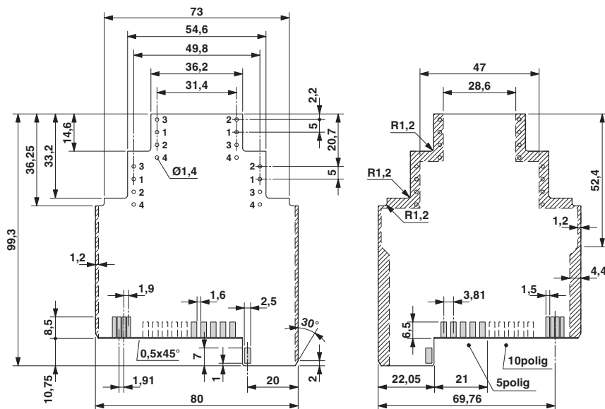
Dimensioned drawing
