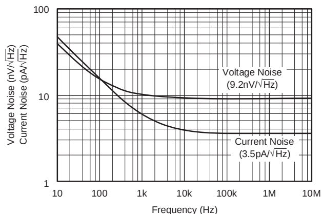
INPUT VOLTAGE AND CURRENT NOISE DENSITY
