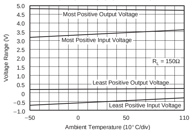
VOLTAGE RANGES vs TEMPERATURE
