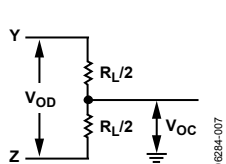
Figure 7. Driver Differential Output Voltage and Common-Mode Output Voltage
