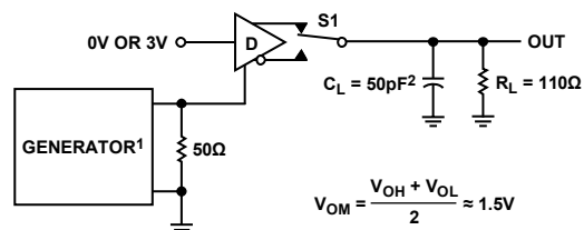
Figure 11. Driver Propagation Delays
