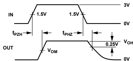
Figure 12. Driver Enable and Disable Times ( t_{PZH} , t_{PSH} , t_{PHZ} )
