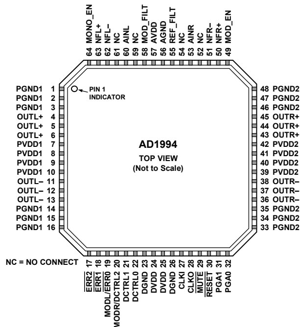
Figure 3. Pin Configuration
