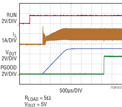
Start-Up With Load in Burst Mode Operation
