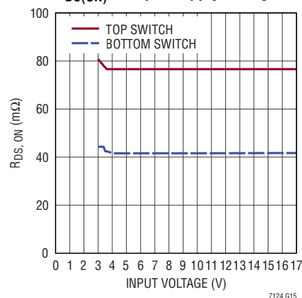
R_{DS(ON)} vs Input Supply Voltage
