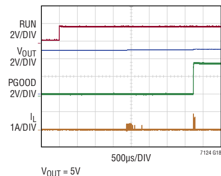
Start-Up into Pre-Biased Output in Burst Mode Operation
