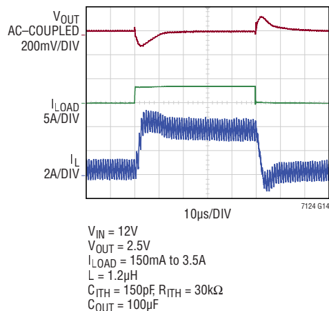
Load Step with External Compensation
