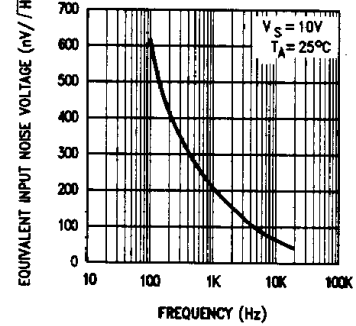
Equivalent Input Noise Voltage of Op-Amps
