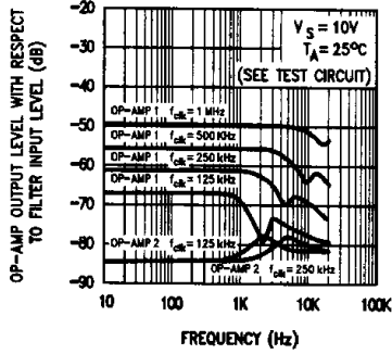
Crosstalk from Filter to Op-Amps (MF6-50)
