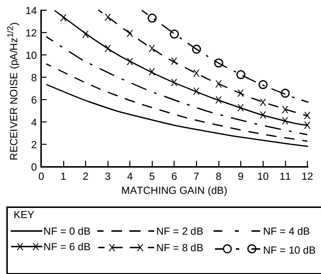
Figure 1. Receiver Noise
