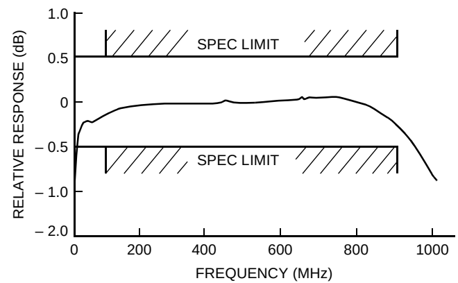
Figure 2. Typical Frequency Response Measured into 75 \Omega Load, VSWR <1.5
