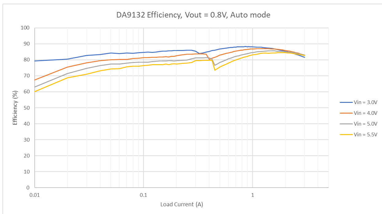
Figure 7: DA9132-A Efficiency, V_{OUT} = 0.8V , Auto Mode
