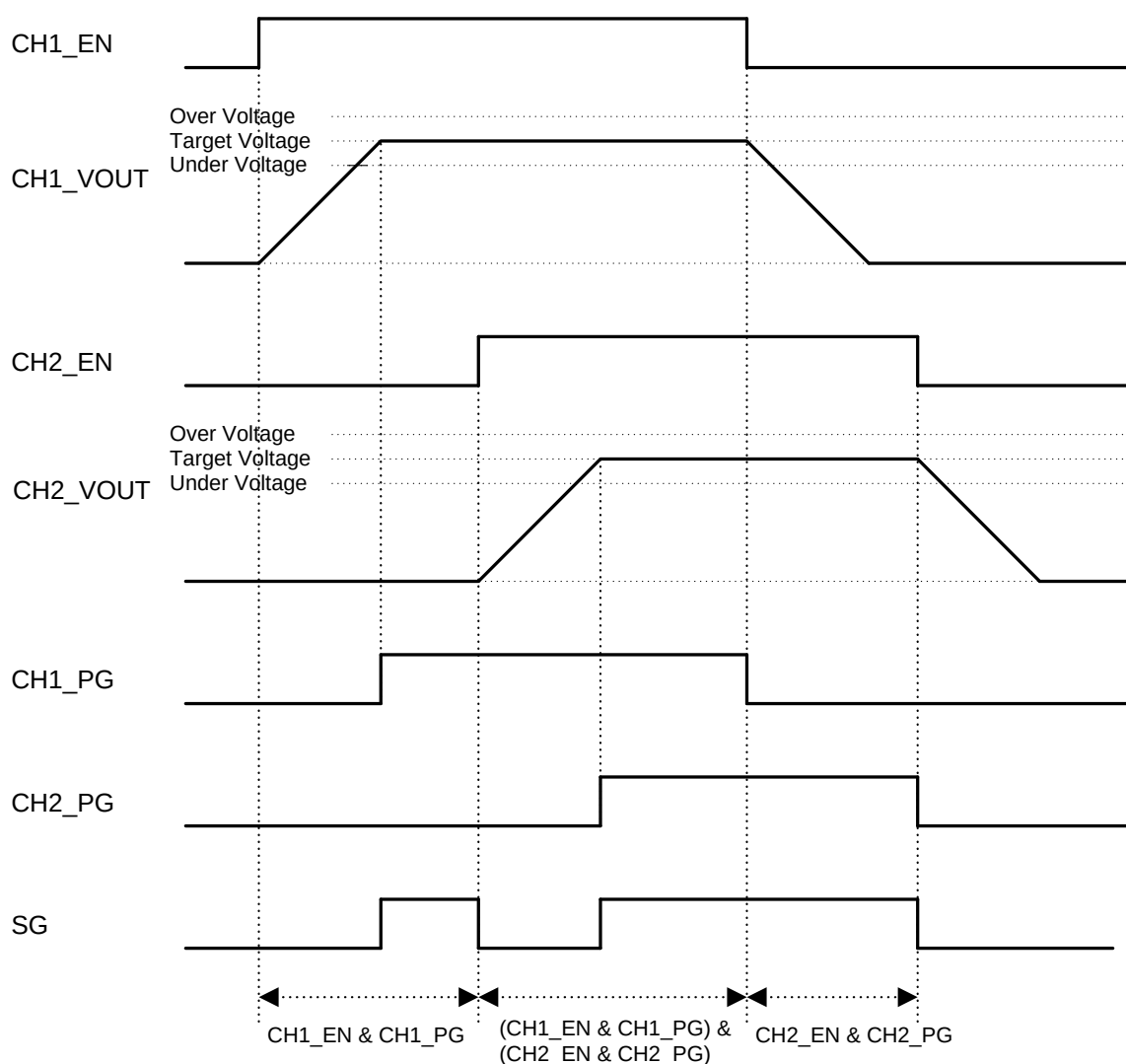
Figure 15: Power-Good (PG) and System Good (SG)
