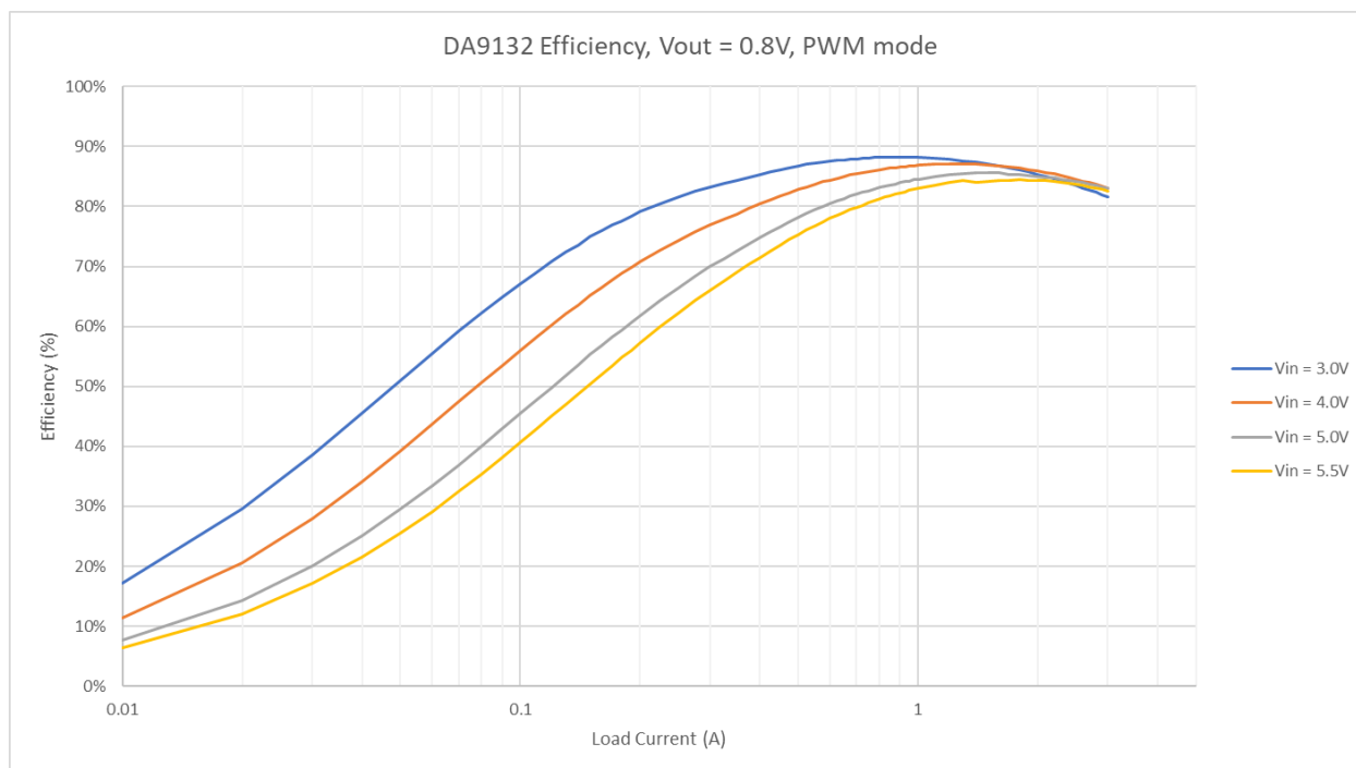
Figure 6: DA9132-A Efficiency, V_{OUT} = 0.8V , PWM Mode
