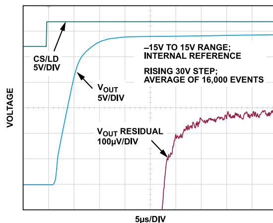
Figure 37. Settling Time, 30 V
