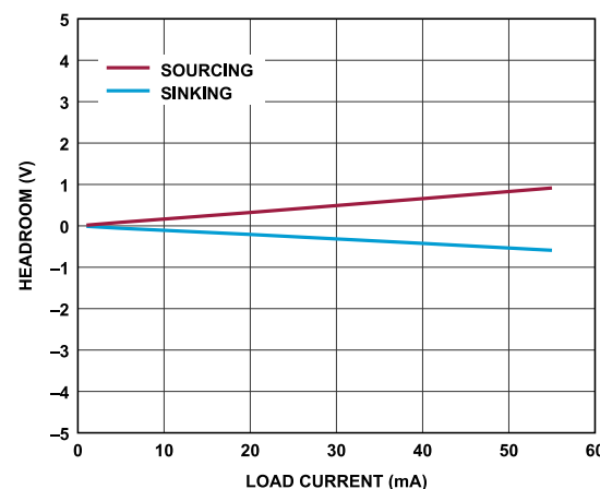
Figure 39. V_{x+}/V_{-} Unipolar Headroom vs. Output Load Current
