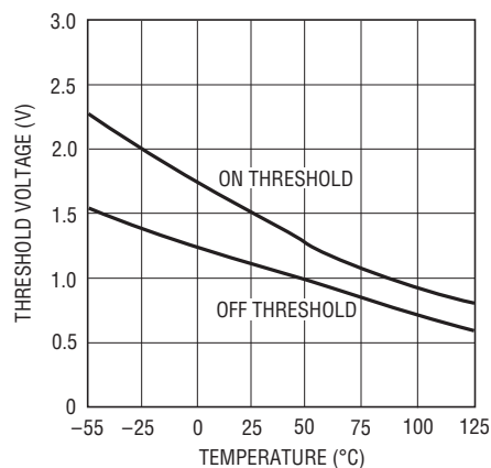
ON/OFF Thresholds
