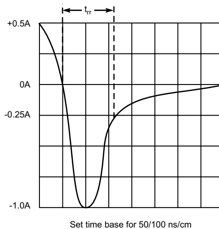
Fig. 5 Reverse Recover Time Characteristic and Test Circuit
