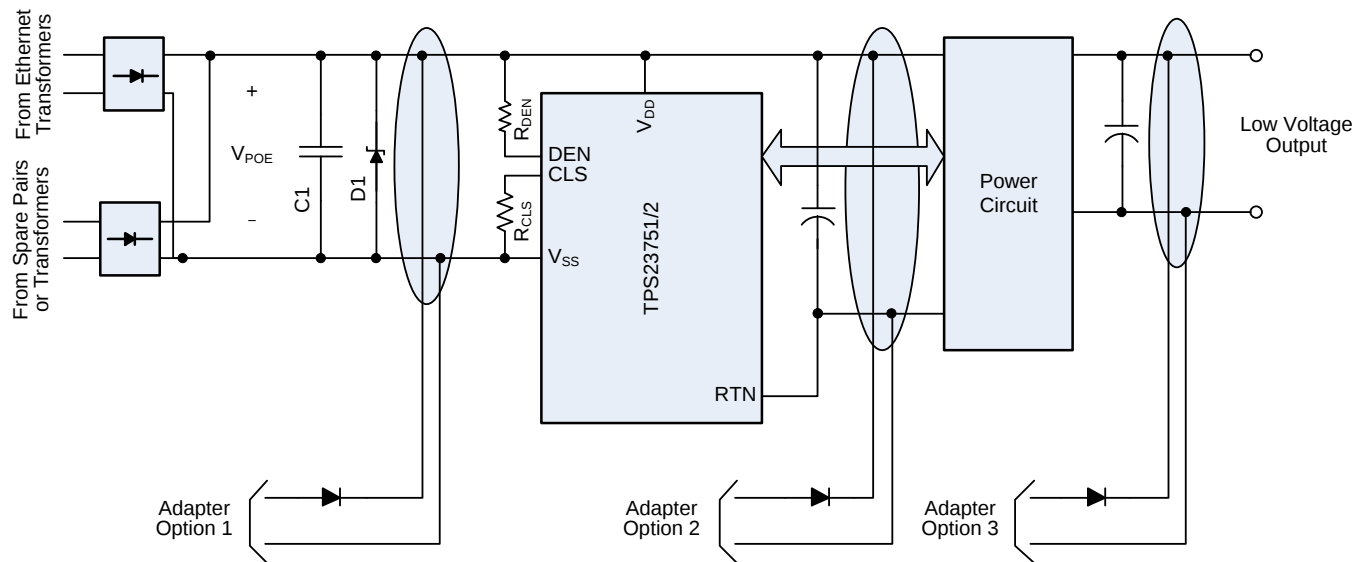
Figure 31. ORing Configurations
