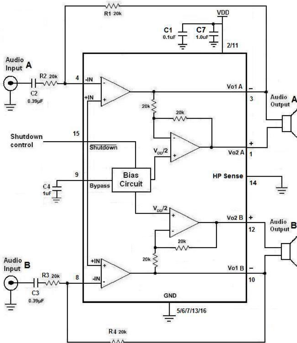
Figure 1. Without Headphone Typical Application Circuit (QFN16)
