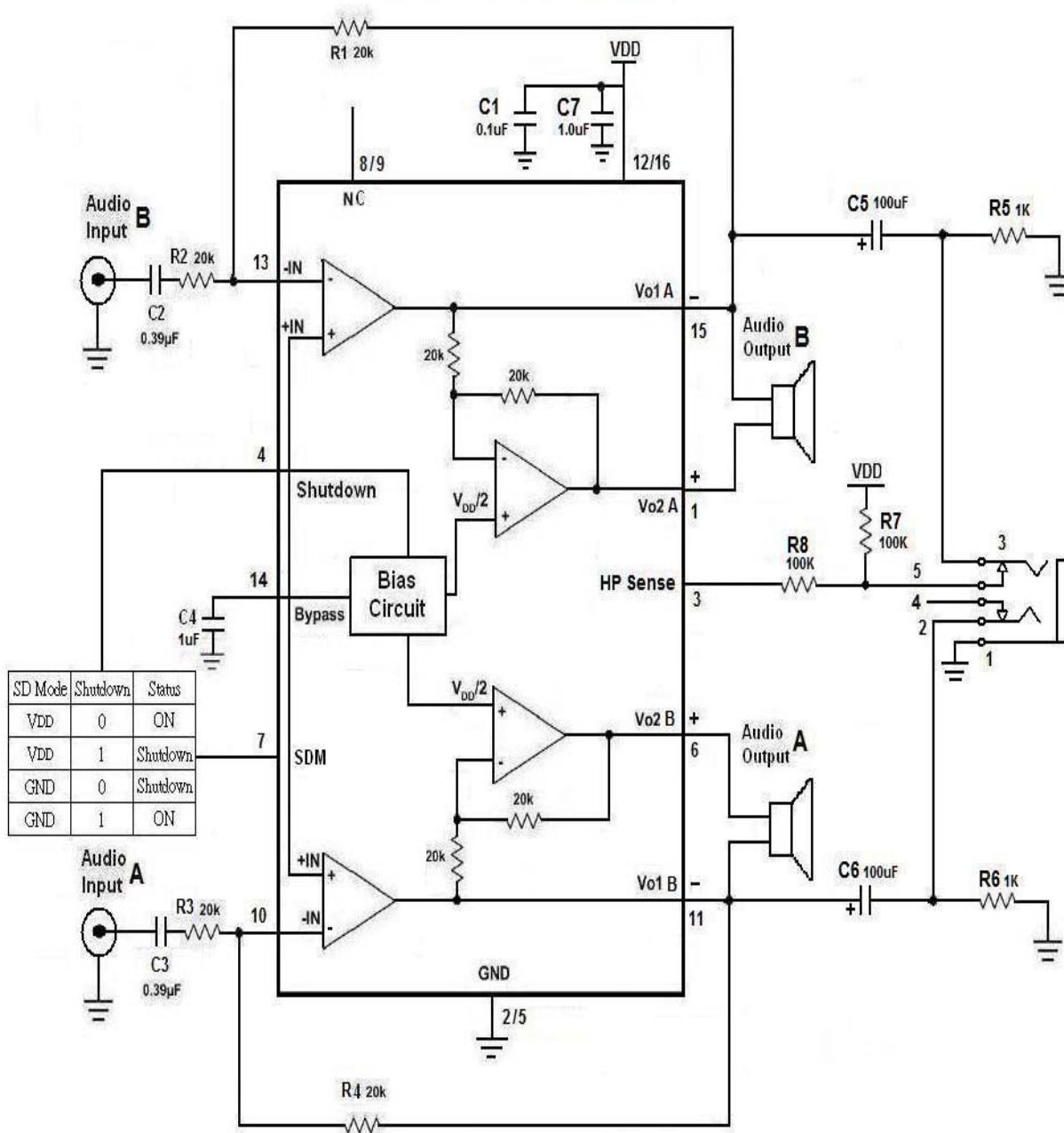
Figure 4. With Headphone Typical Application Circuit (SOP16)
