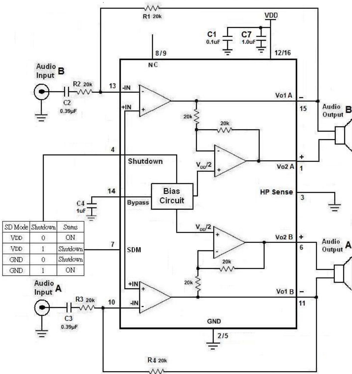
Figure 3. Without Headphone Typical Application Circuit (SOP16)
