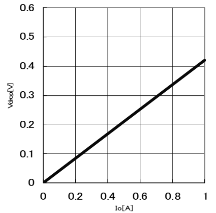
Fig.21 Minimum dropout Voltage 3 (Vcc=6V, Ta=25°C)
