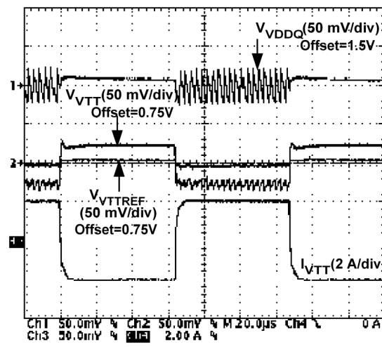
图 7-23. VTT Load Transient Response
