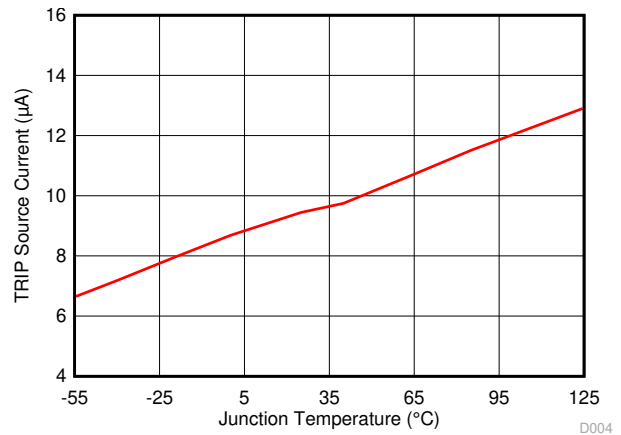
图 7-5. Current Sense Current vs Junction Temperature
