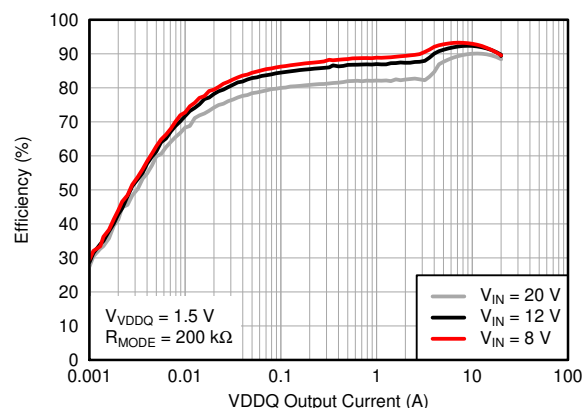
图 7-21. Efficiency
