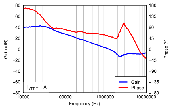
图 7-29. VTT Bode Plot (Source)
