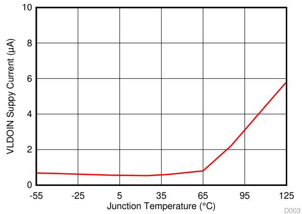
图 7-4. VLDOIN Supply Current vs Junction Temperature
