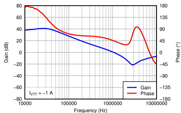
图 7-28. VTT Bode Plot (Sink)
