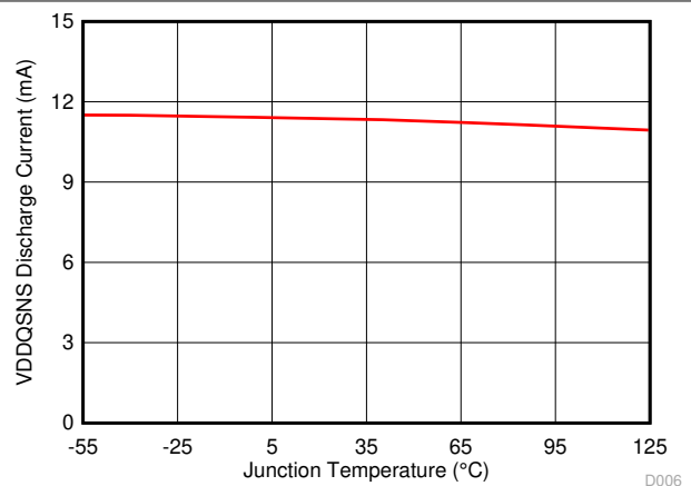
图 7-7. VDDQSNS Discharge Current vs Junction Temperature
