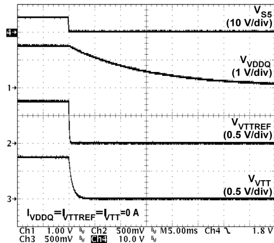
图 7-27. 1.5-V Soft-Stop Waveforms (Non-Tracking Discharge)
