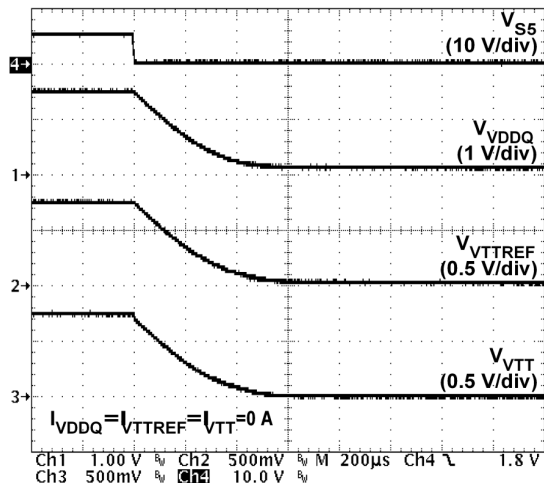
图 7-26. 1.5-V Soft-Stop Waveforms (Tracking Discharge)
