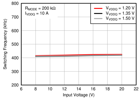
图 7-10. Switching Frequency vs Input Voltage
