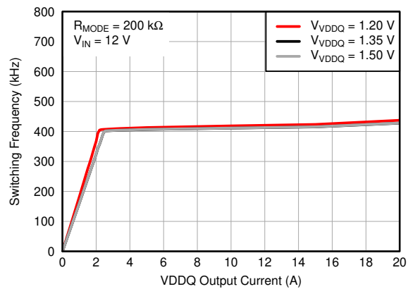
图 7-12. Switching Frequency vs Load Current
