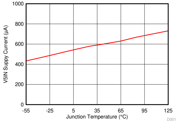
图 7-2. V5IN Supply Current vs Junction Temperature
