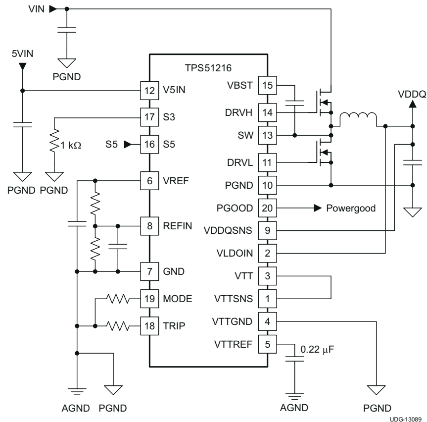
图 9-3. Application Circuit When VTT is not Required
