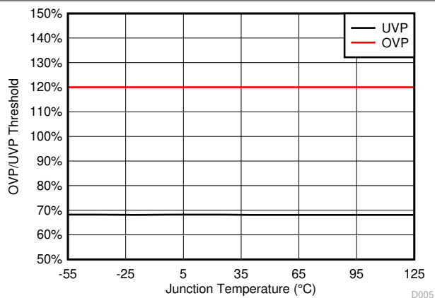
图 7-6. OVP/UVP Threshold vs Junction Temperature
