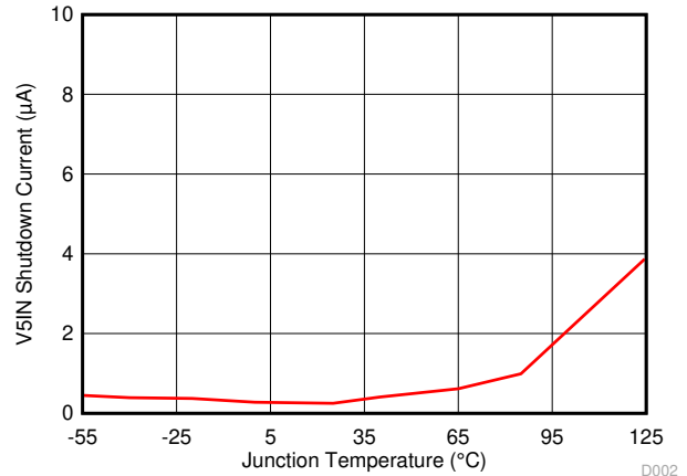
图 7-3. V5IN Shutdown Current vs Junction Temperature
