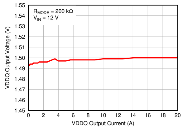
图 7-13. Load Regulation
