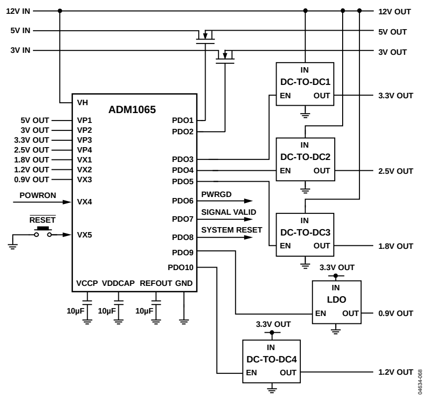
Figure 24. Applications Diagram
