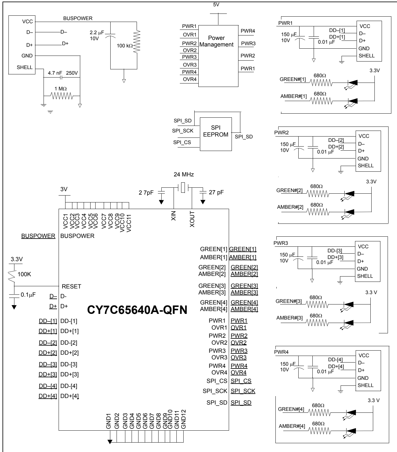
Figure 13-1. Sample Schematic
