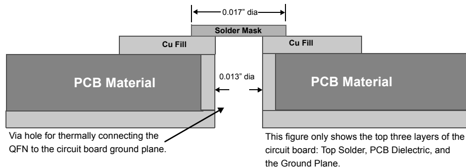
Figure 16-2. Cross section of the Area Underneath the QFN Package
