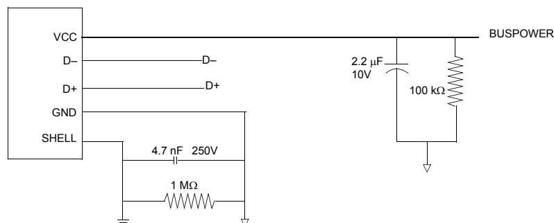
Figure 10-1. USB Upstream Port Connection
