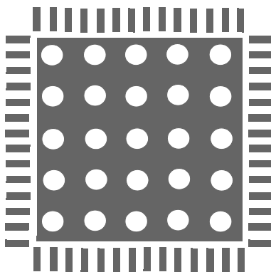
Figure 16-3a. Plot of the Solder Mask (White Area)
