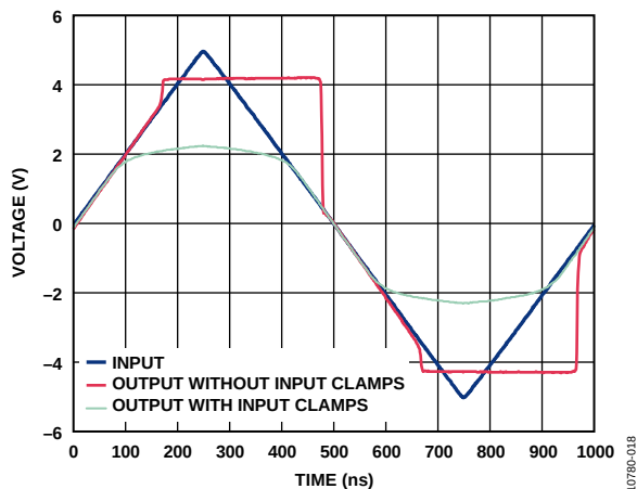
Figure 18. Overdrive Recovery, G = 1
