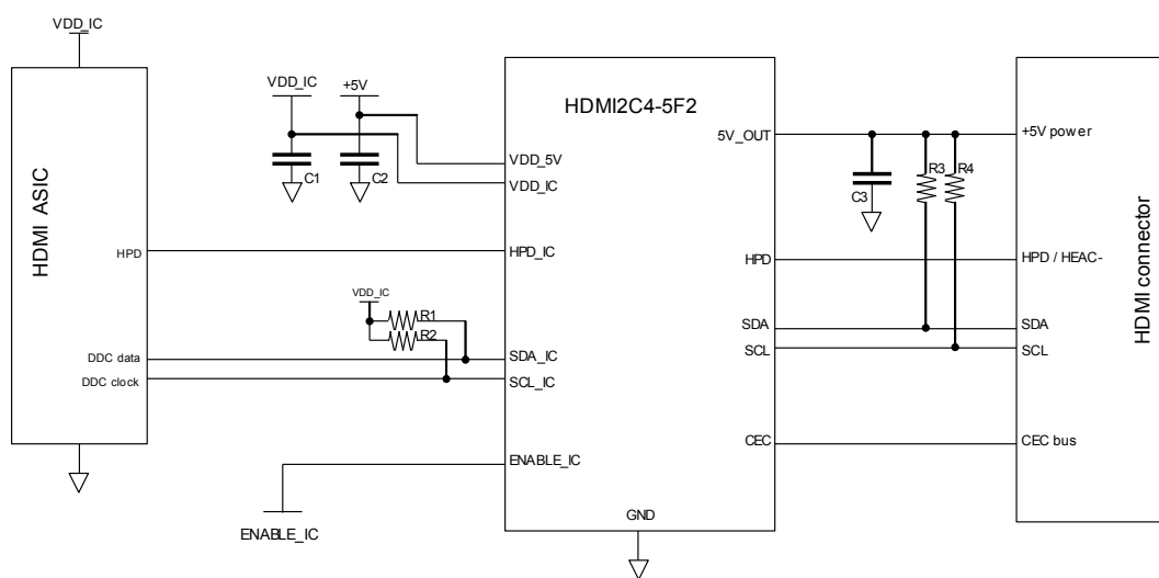
Figure 9. Application block diagram
