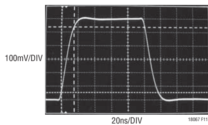
Figure 11. Step Response with R_F = 499\text{k}
