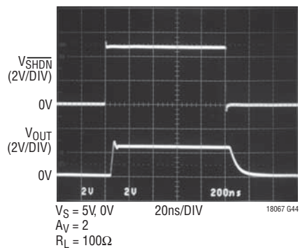
Shutdown Response
