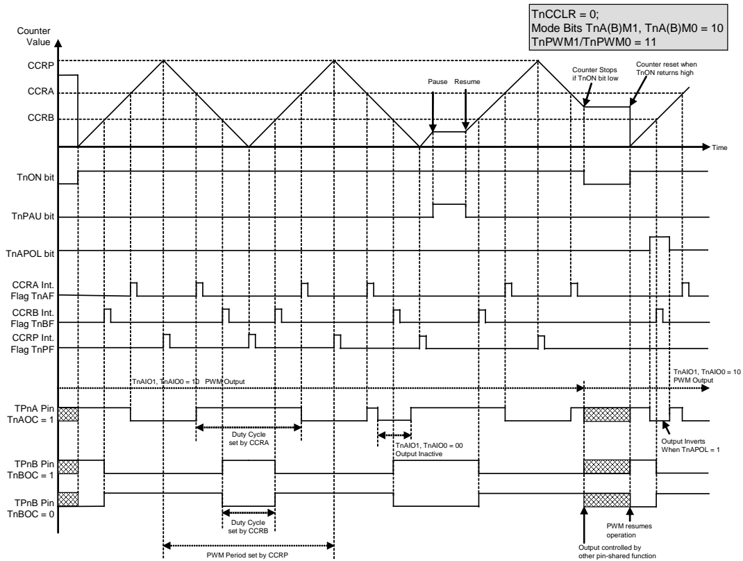
ETM PWM Mode – Centre Aligned
