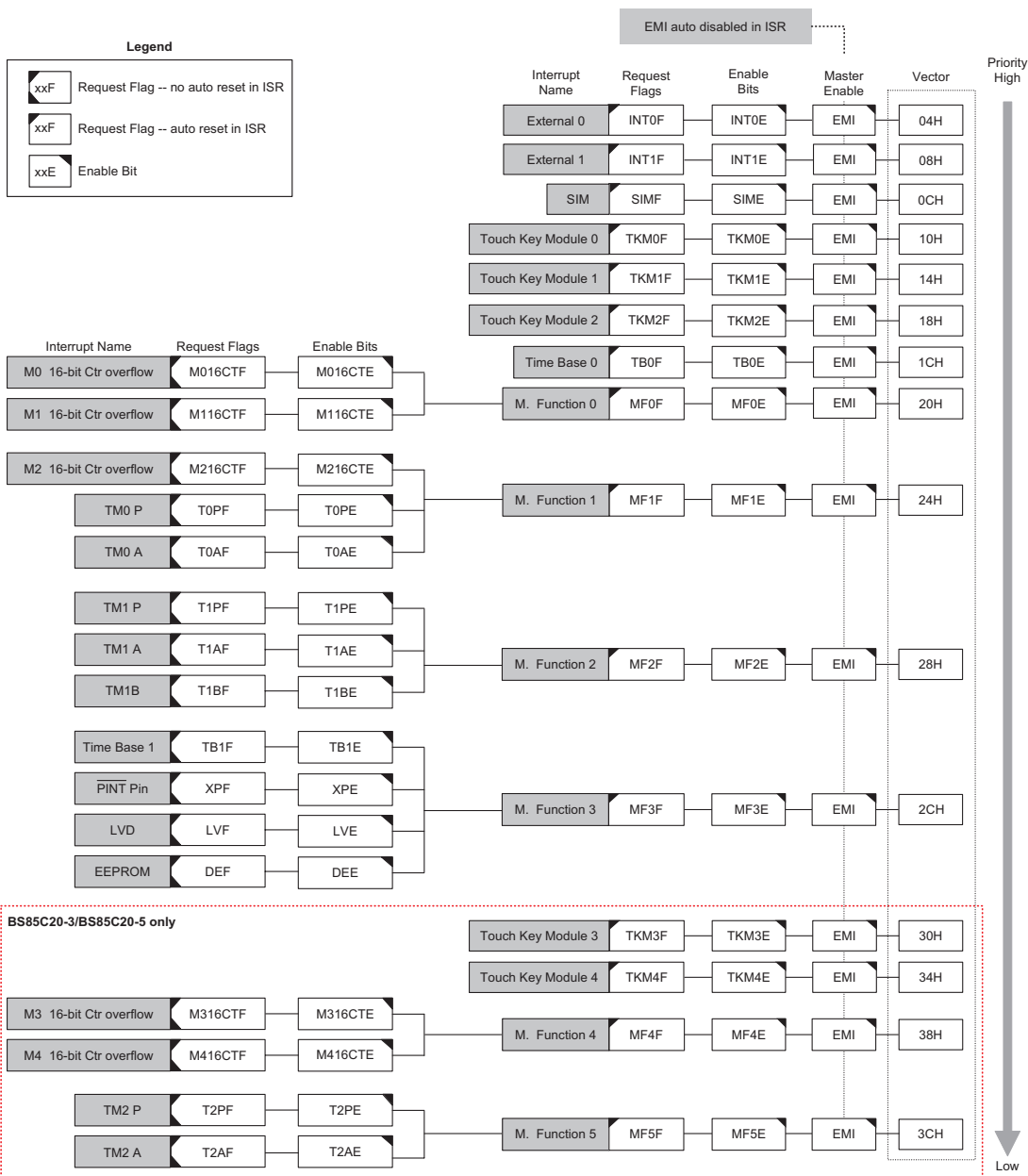
Interrupt Structure
