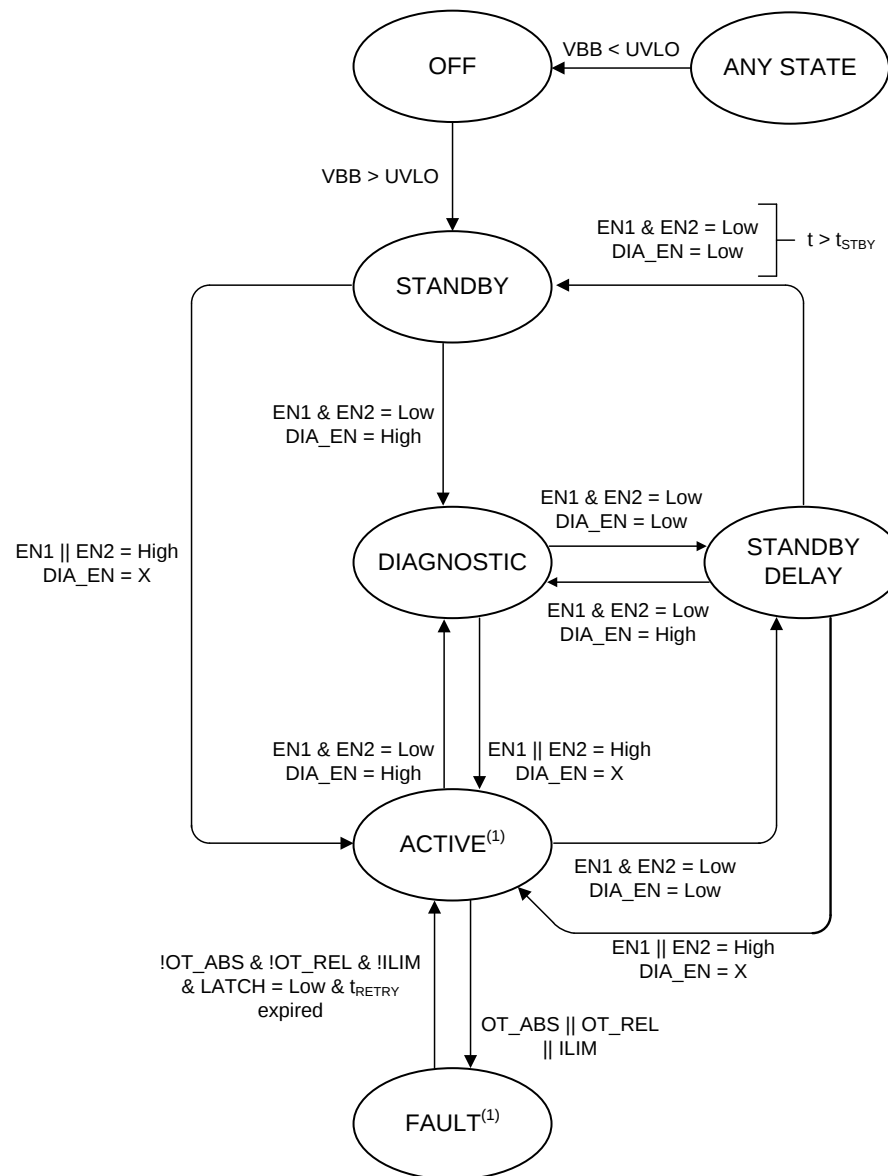
Figure 14. State Diagram
