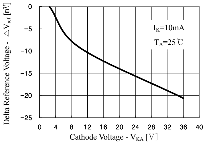
Fig.9 \Delta V_{ref} vs V_{KA}
