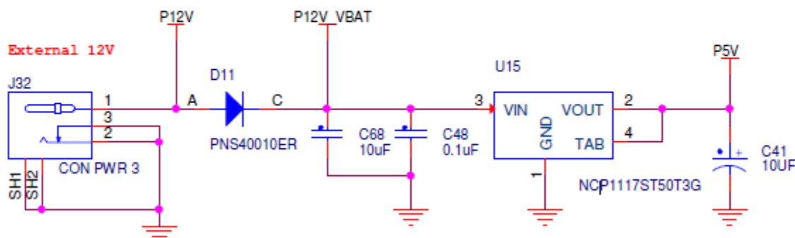
Figure 24. CAN power circuit
