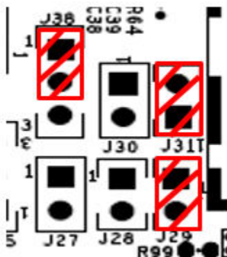
Figure 16. Jumper settings for Buck mode (manual start)
