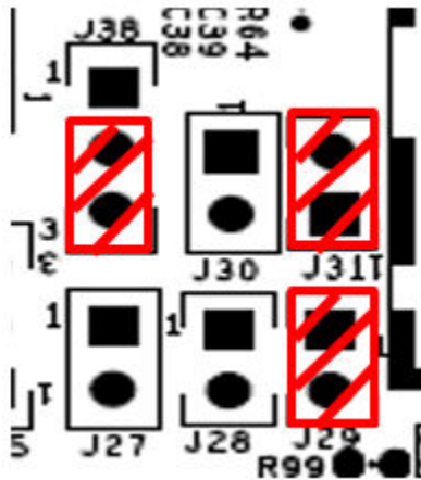
Figure 17. Jumper settings for Buck mode (auto start)
