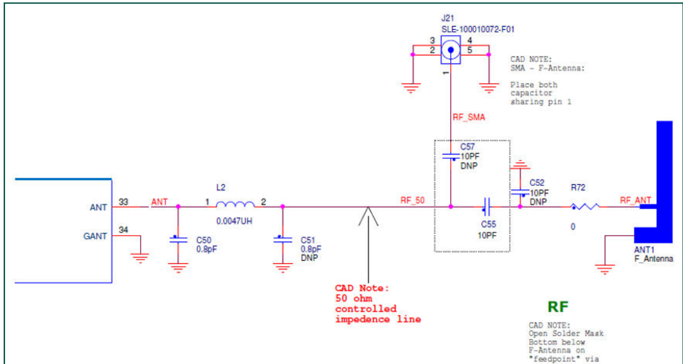
Figure 5. FRDM-KW36 RF circuit - 2 components
