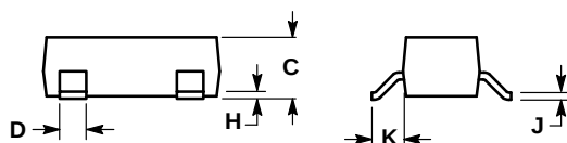
CASE 318-08 ISSUE AE SOT-23 (TO-236AB)
