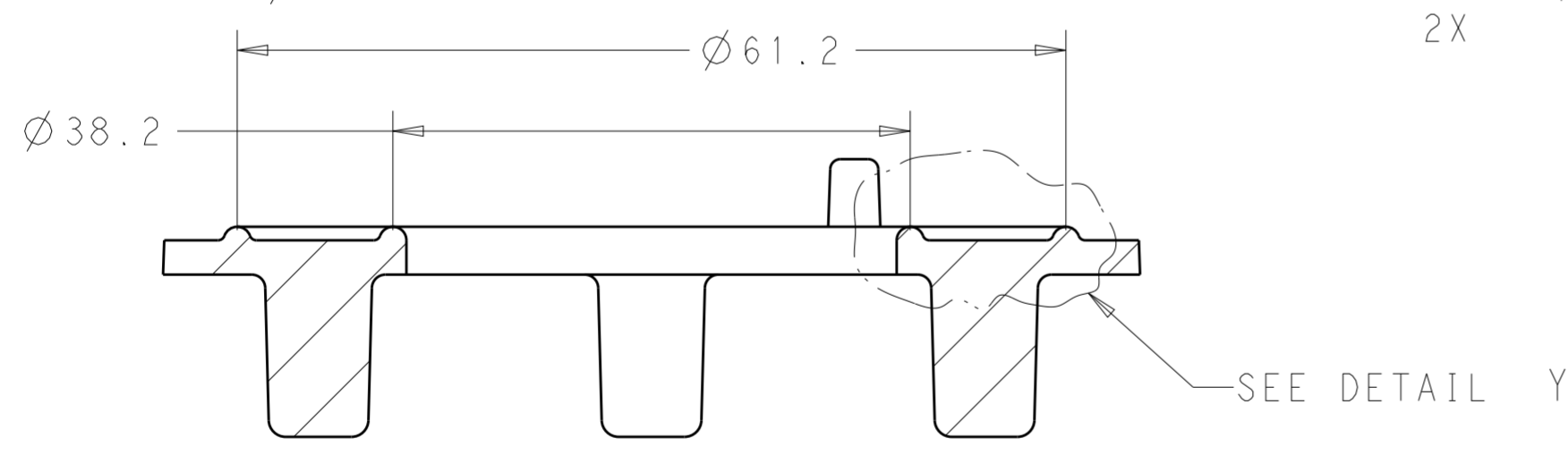
SECTION X-X
