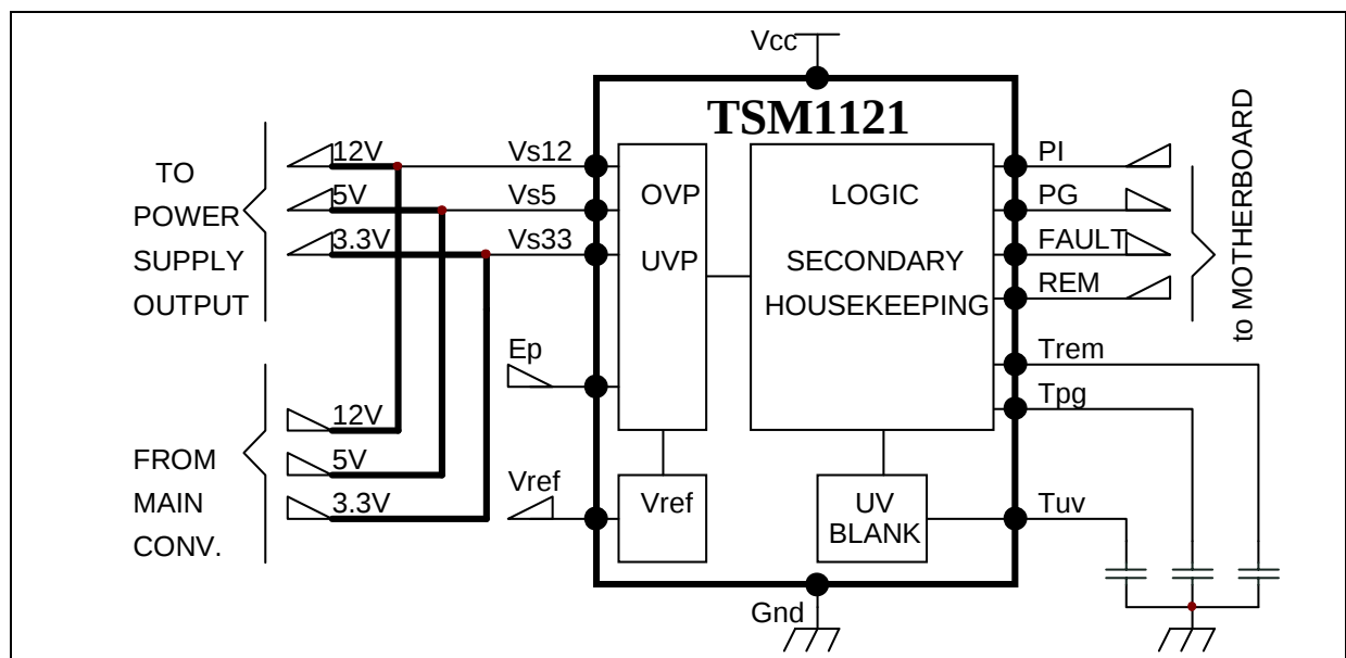
Fig. 2: Internal Schematic
