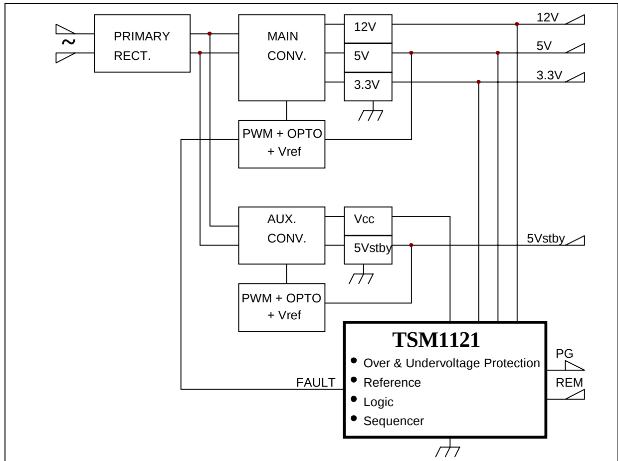
Fig. 2: Internal Schematic
