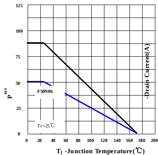
Figure.9 Power Dissipation
