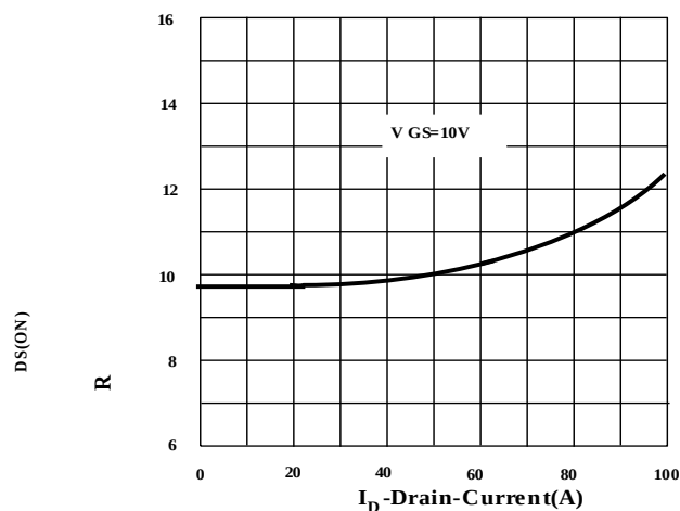
Figure.2 Drain- Source On Resistance
