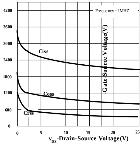
Figure.7 Capacitance
