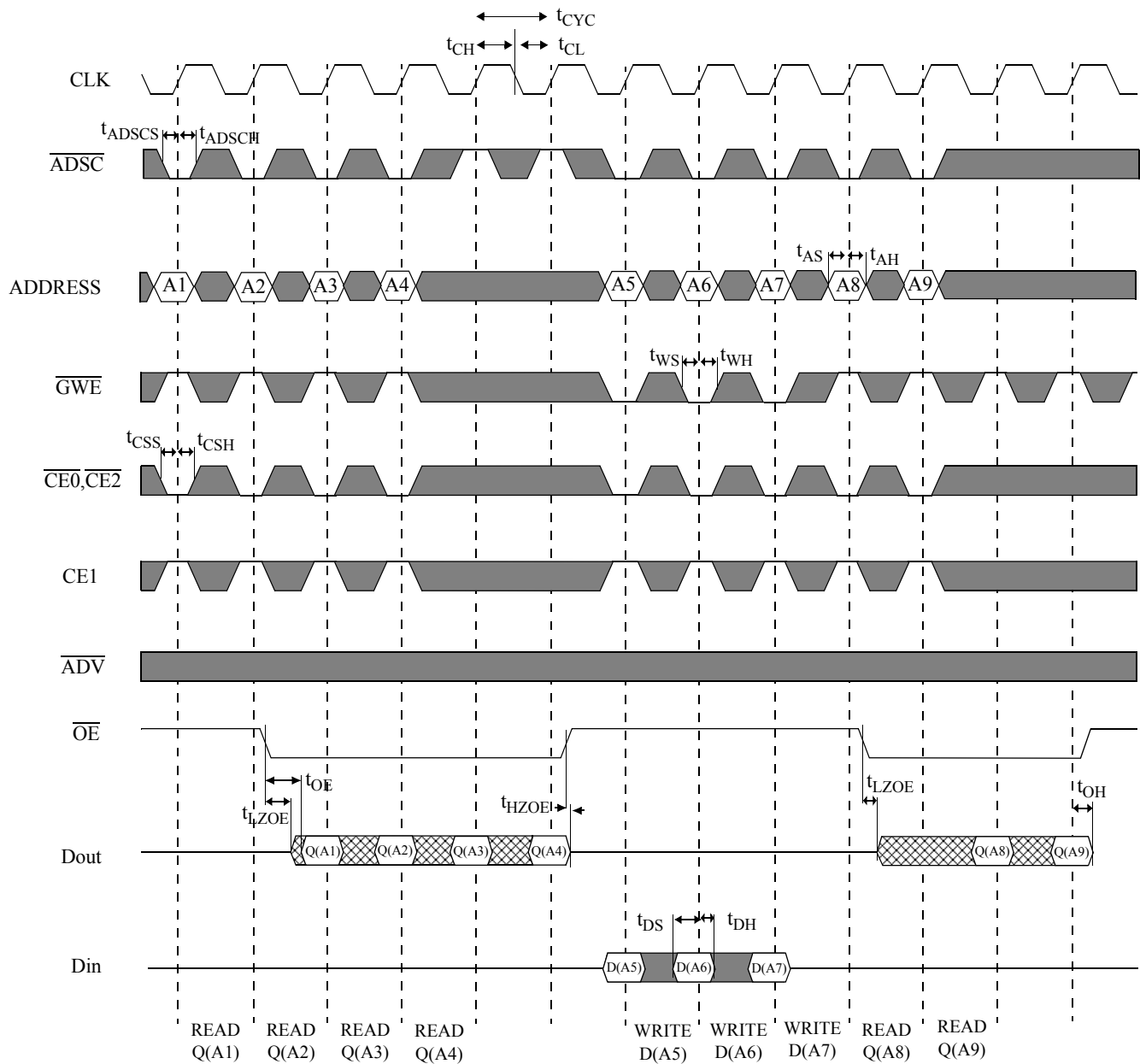
Timing waveform of read/write cycle ( \overline{\text{ADSC}} controlled, \overline{\text{ADSP}} = \text{HIGH} )
