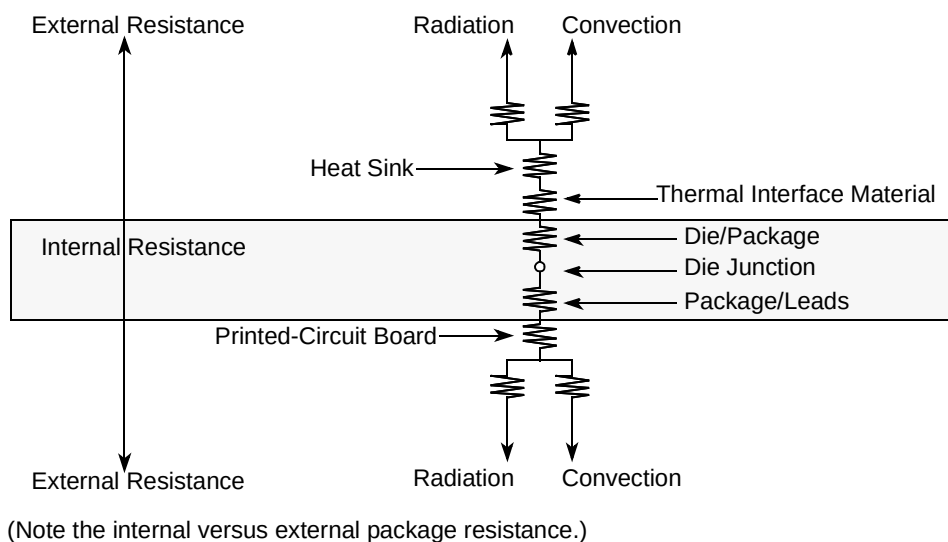
Figure 28. TBGA Package with Heat Sink Mounted to a Printed-Circuit Board
