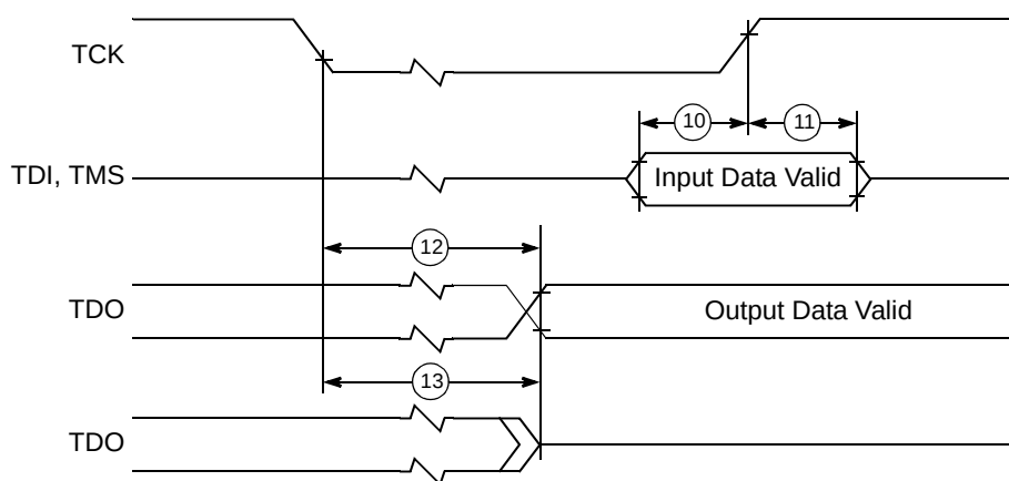
Figure 22. Test Access Port Timing Diagram
