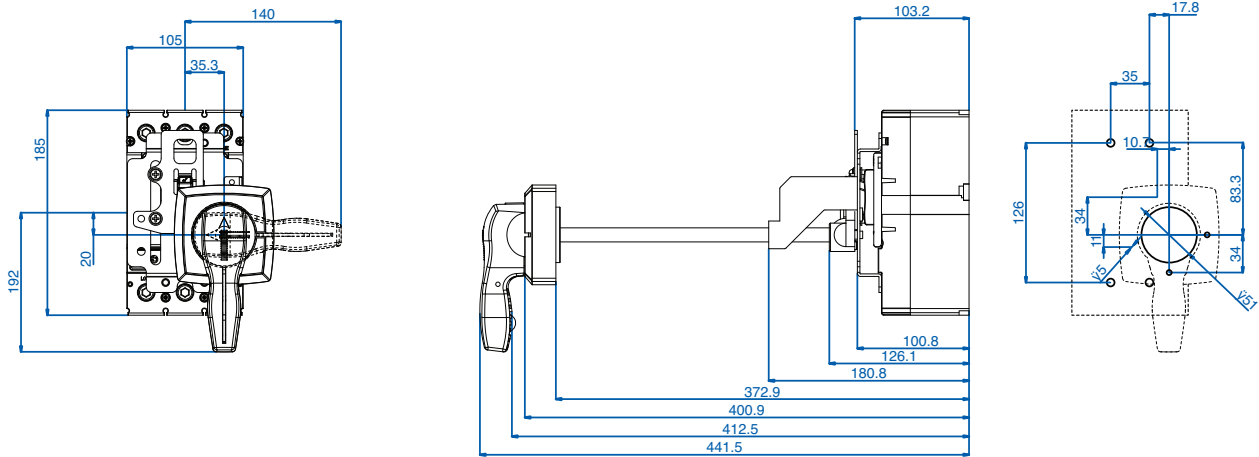
ABS-,ABH-,ABL-403U handle
