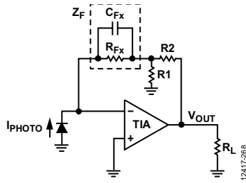
图71. T网络
