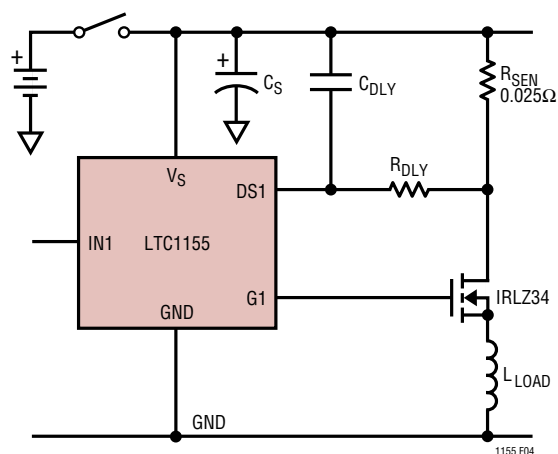
Figure 4. Switched Supply
