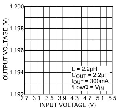
Line Regulation
