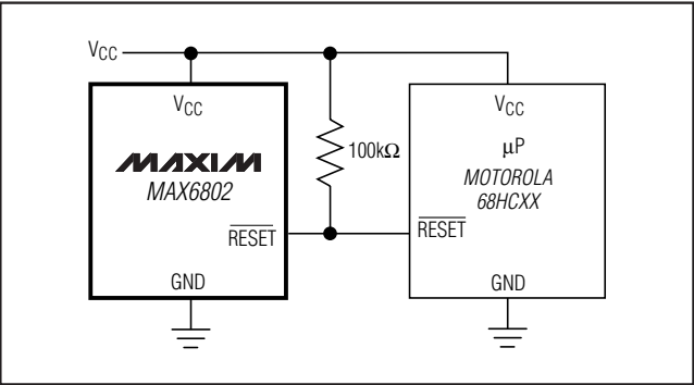
Figure 1. Interfacing to μPs with Bidirectional Reset Pins
