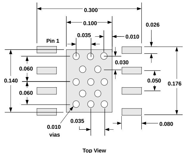
Figure 67. DDA PowerPAD PCB Etch and Via Pattern
