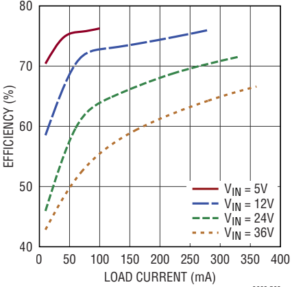
Efficiency vs Load Current, V_{OUT1} = 3.3\text{V}
