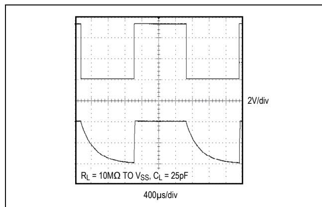
Figure 4. Shutdown Waveform
