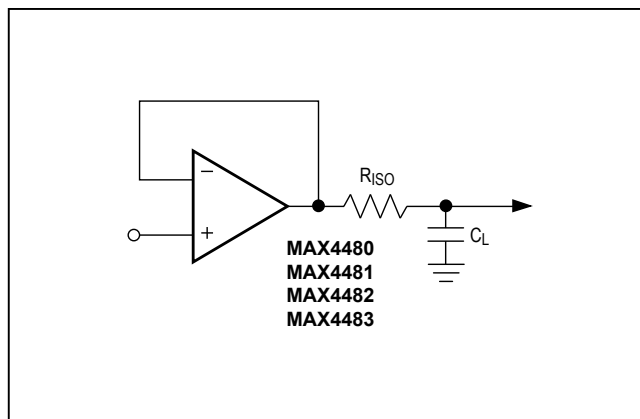
Figure 3. Capacitive-Load-Driving Circuit
