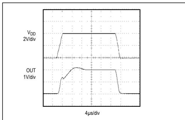
Figure 5. Power-Up/Down Waveform
