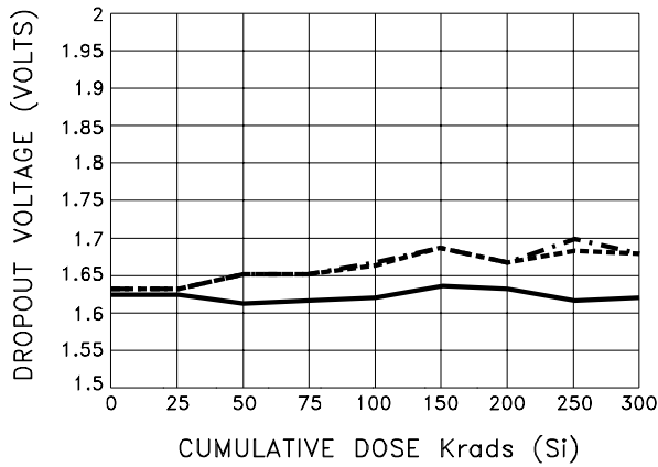
POSITIVE DROPOUT VOLTAGE
