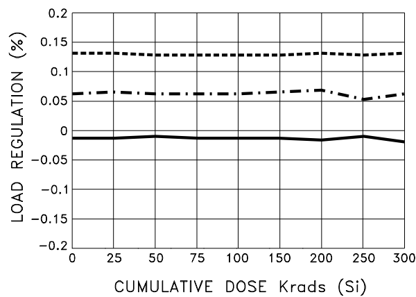
POSITIVE LOAD REGULATION
