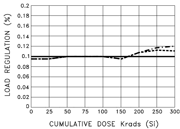
NEGATIVE LOAD REGULATION
