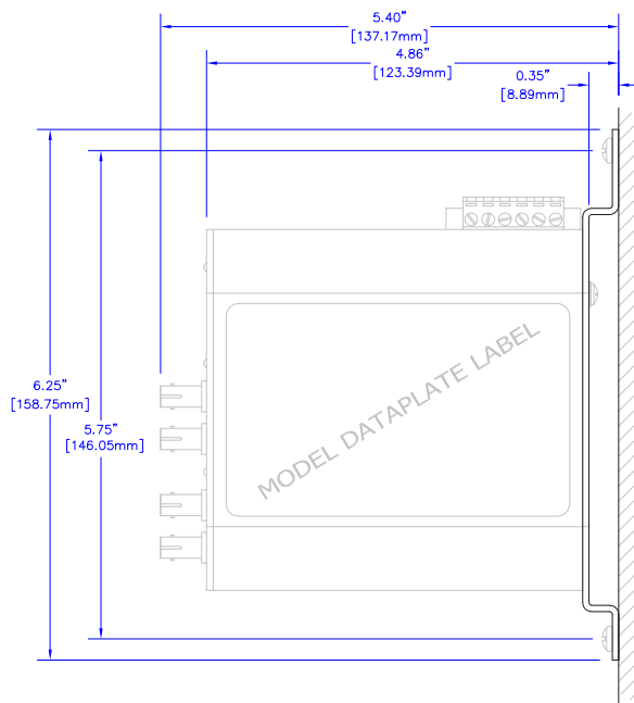
OPTIONAL COMPACT PANEL MOUNT ASSY. ( P/N: CPMA-2 )
