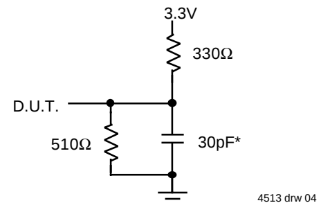
Figure 2. Output Load
