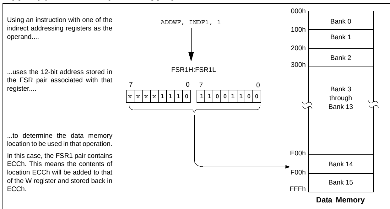
FIGURE 5-9: INDIRECT ADDRESSING
