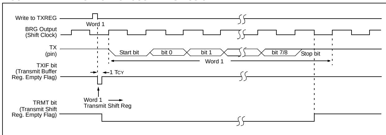
FIGURE 17-4: ASYNCHRONOUS TRANSMISSION
