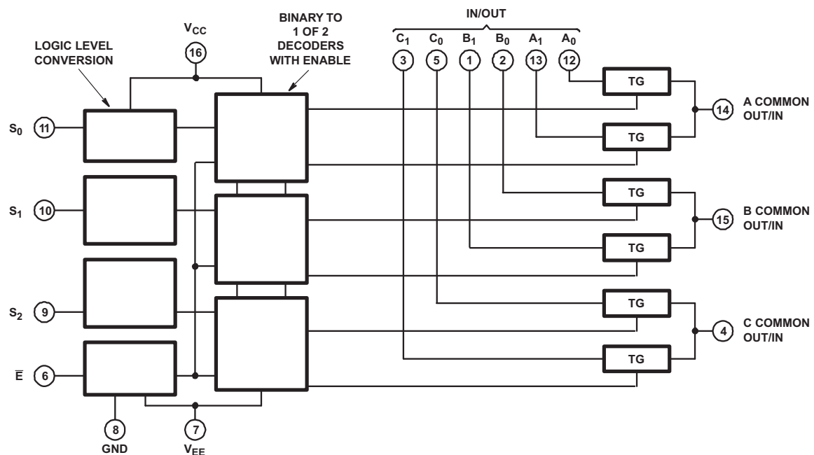
Figure 19. CDx4HCx4053 Functional Block Diagram
