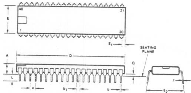
40-Pin Molded DIP
