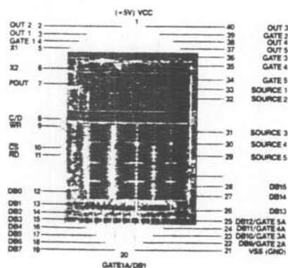
Metallization and Pad Layout
