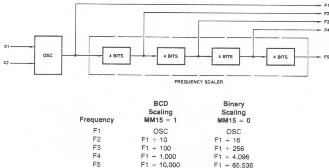
Figure 16. Frequency Scaler Ratios.
