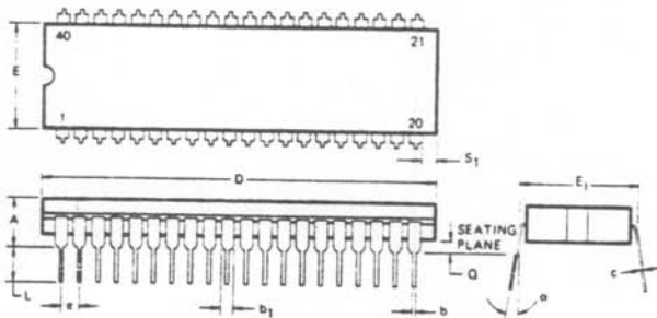
40-Pin Cerdip
