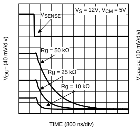
Figure 12. Settling Time (Fall)
