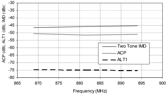
Two Tone IMD, ACP, ALT1 vs. Frequency Output Power=1 Watt, Vdd=28 V, T Flange =25°C IS95 standard, channel BW= 1.23 MHz, ADJ BW= 30 KHz@ 750 KHz spacing. ALT1 BW= 30 KHz@1980 KHz spacing. IMD@1 MHz spacing.
