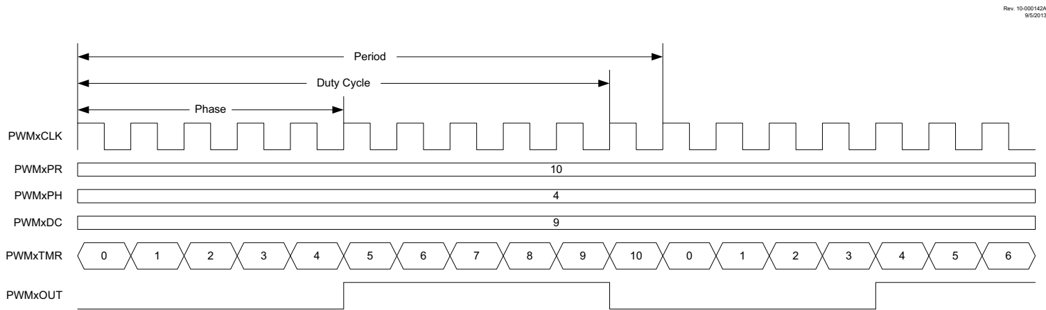
FIGURE 26-4: STANDARD PWMx MODE TIMING DIAGRAM
