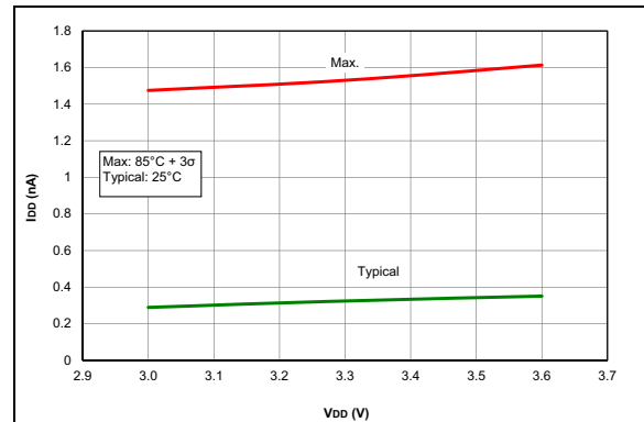
FIGURE 37-35: I_{DD} , LP Brown-Out Reset ( LPBOR = 0 ), PIC16LF1764/5/8/9 Only.
