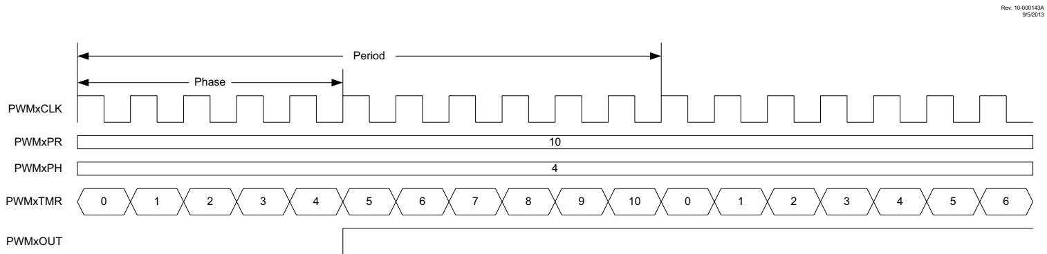
FIGURE 26-5: SET ON MATCH PWMx MODE TIMING DIAGRAM
