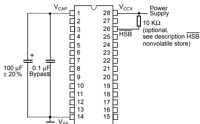
Figure 1: Automatic STORE Operation Schematic Diagram
