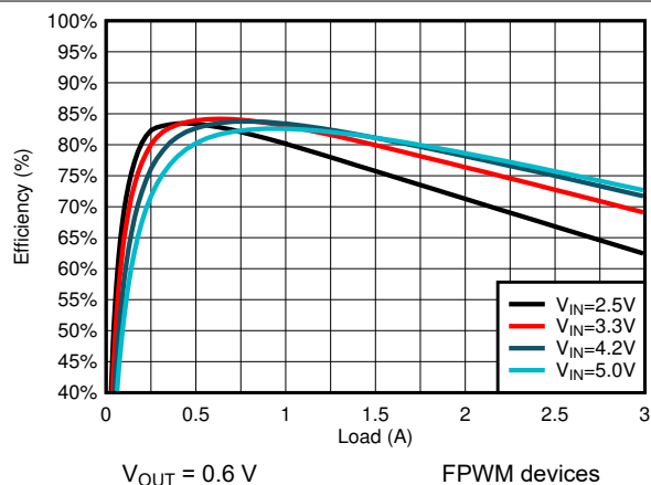
图 9-5. Efficiency
