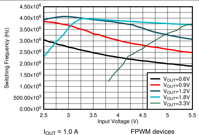
图 9-26. Switching Frequency
