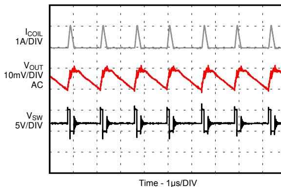
图 9-28. PSM Operation
