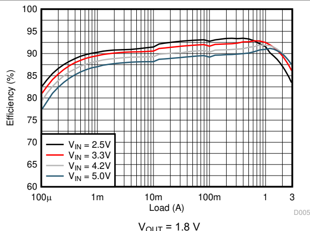
图 9-15. Efficiency
