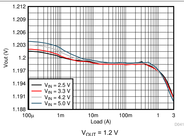
图 9-12. Load Regulation
