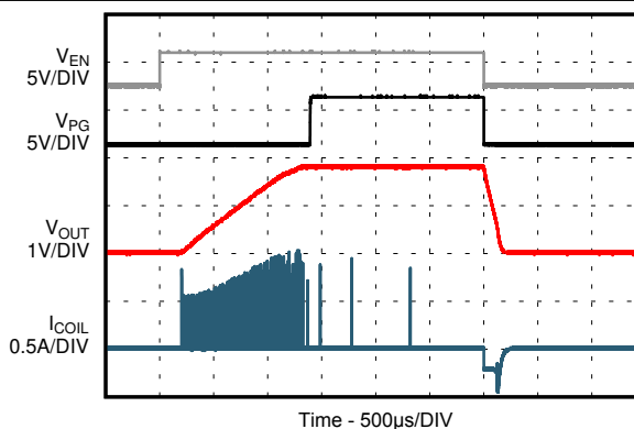
图 9-28. PSM Operation
