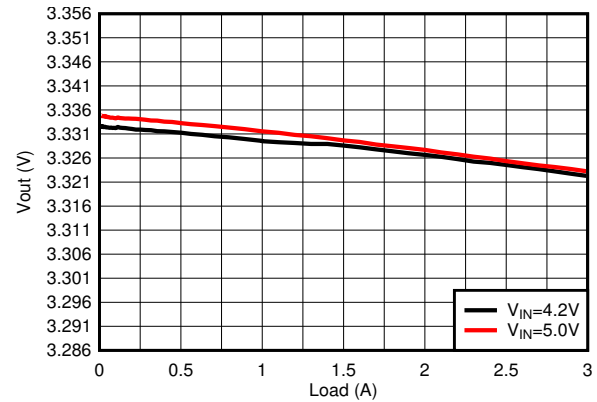
图 9-22. Load Regulation
