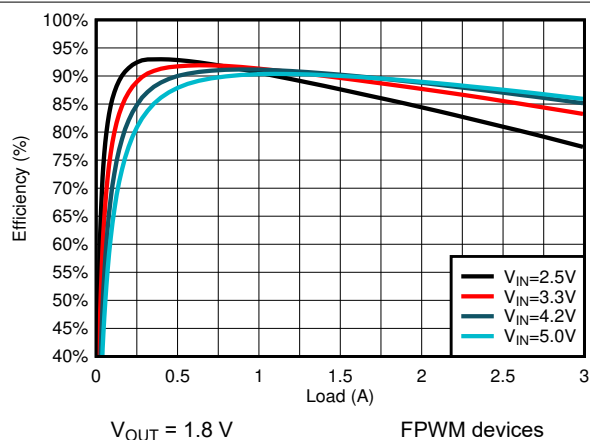
图 9-17. Efficiency
