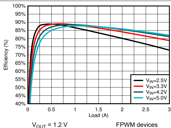
图 9-13. Efficiency
