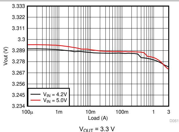
图 9-20. Load Regulation
