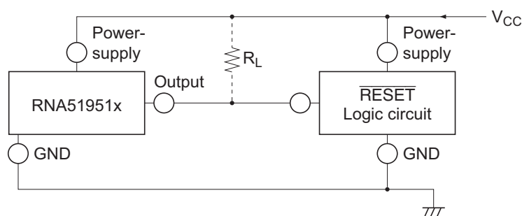
Figure 1 Reset Circuit of RNA51951
